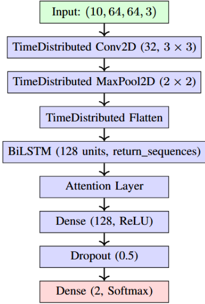
Fig. 3. Block diagram of the Tier 3 CNN-BiLSTM-Attention model architecture.
