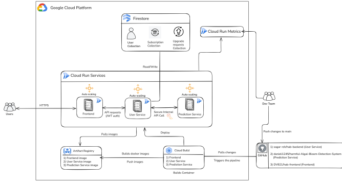
Fig. 1. Deployment architecture on GCP with CI/CD and managed services.
