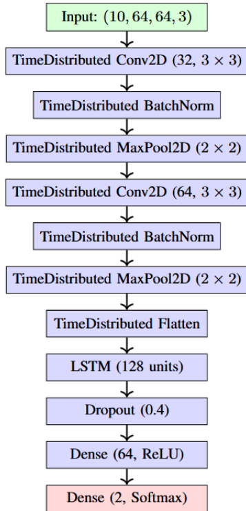
Fig. 2. Block diagram of the Tier 2 CNN-LSTM spatio-temporal network architecture.
